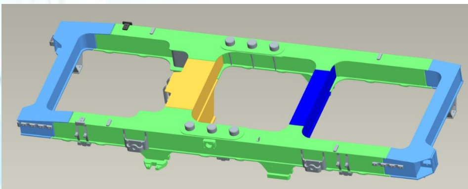
1-rasm. “20‘ZELR” seriyali magistral elektrovoz aravacha ramasi
